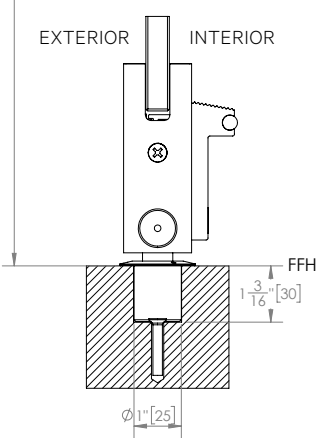
Adjustable Eccentric Floor Socket
