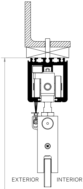
Head Track with L-Bracket
