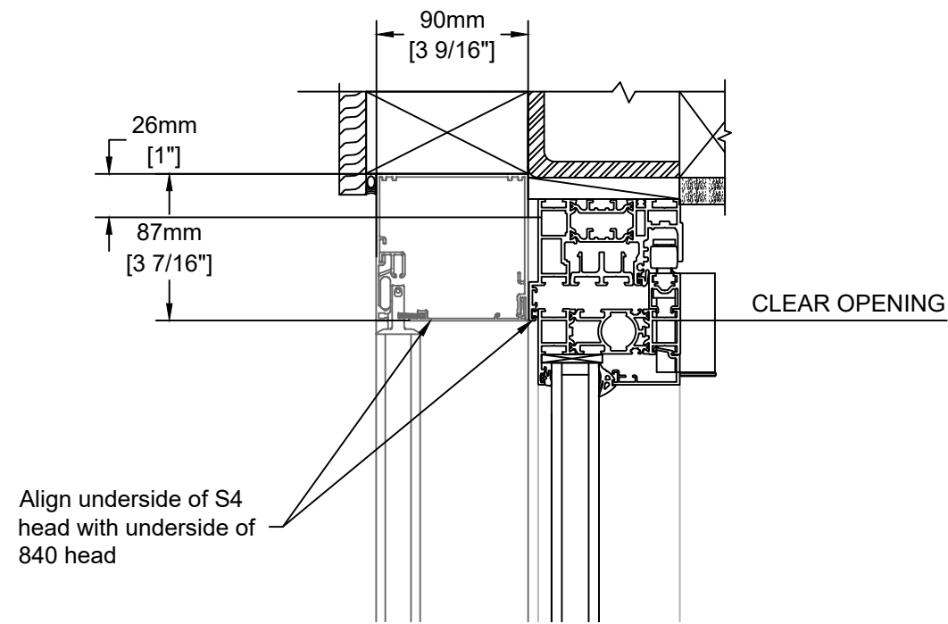
Vertical Section - Head
