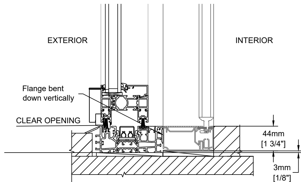
Vertical Section - Sill
