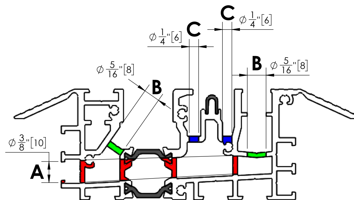
Low Profile Saddle Sill Option 1 Detail Drawing
