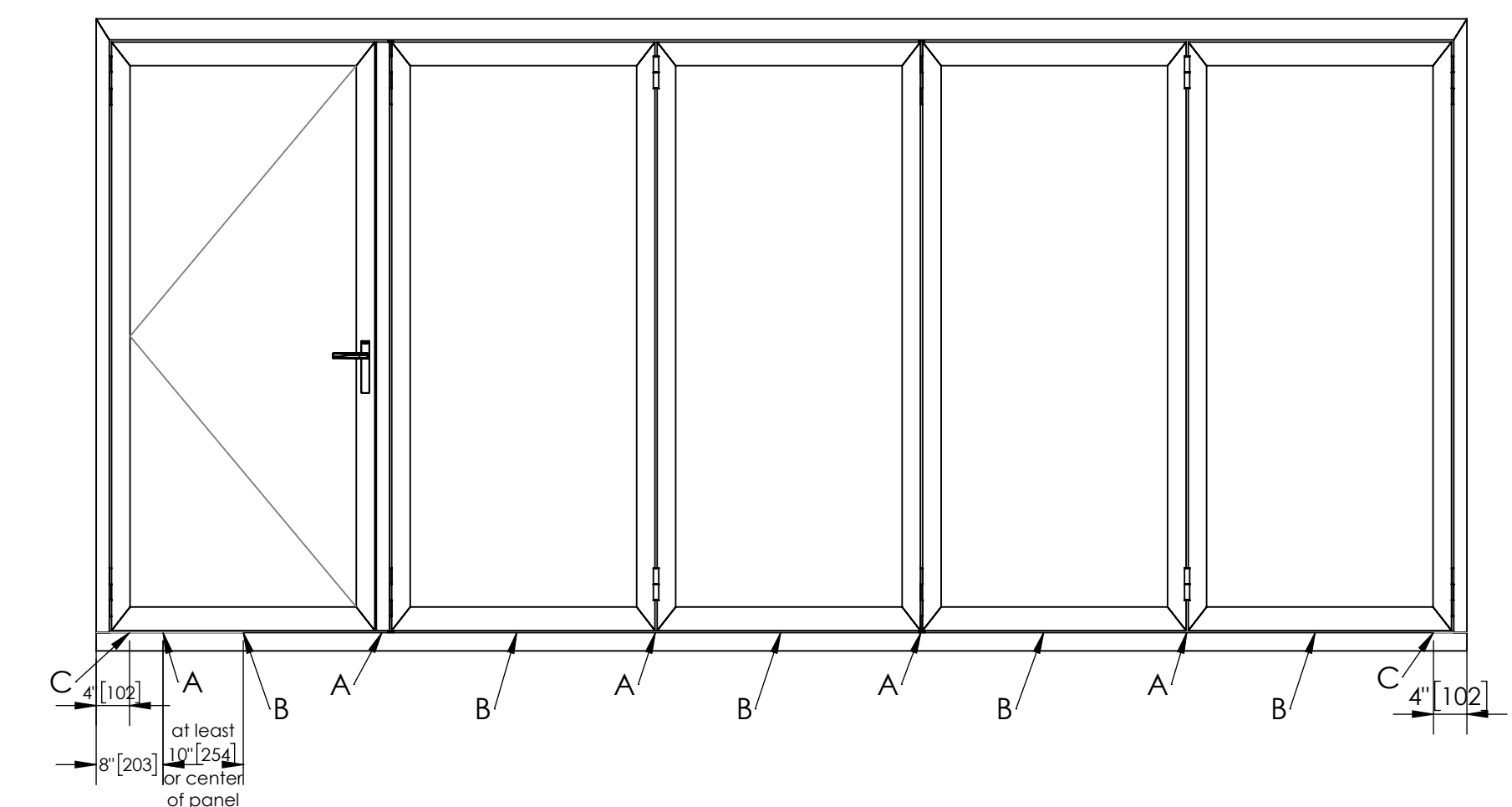
Location of various holes per the Low Profile Saddle Sill Option 1 Drawing
