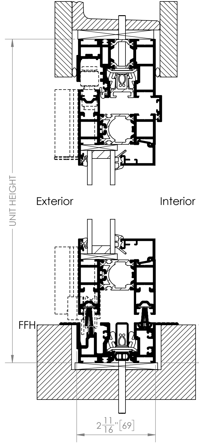
Flush Sill
