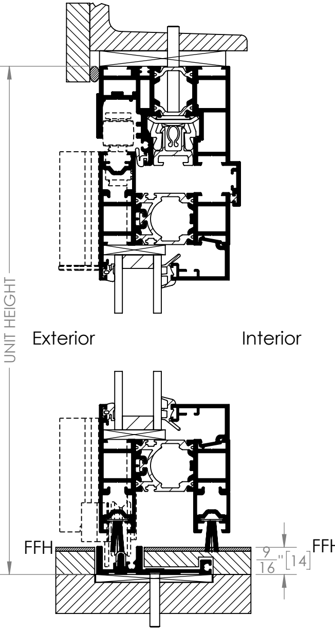
Head Track
