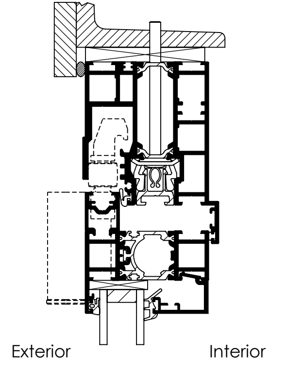
Head Track for Left/Right FourFold and SixFold Panel Sets
