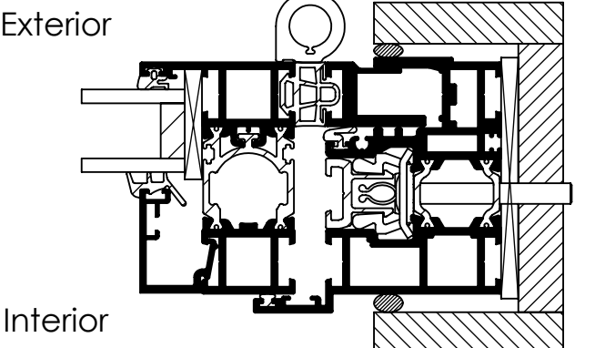
Panel Hinged at Right with Recessed Side Jamb
